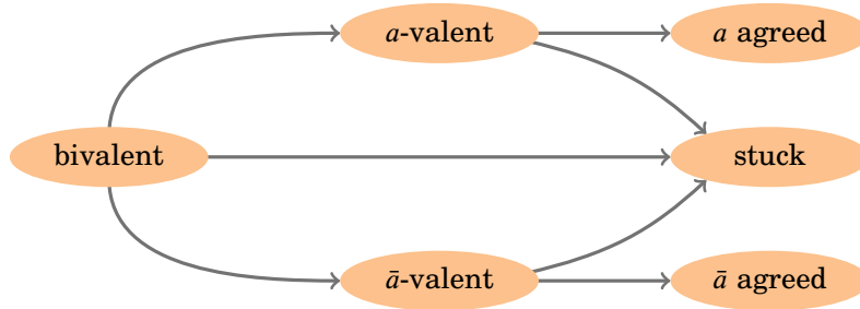
Fig. 12. Possible system-wide status of a statement a
